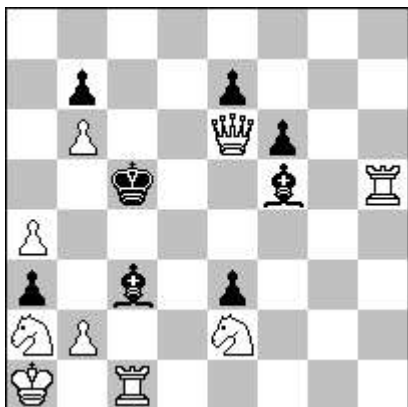
s # 7* v (9 + 8)
