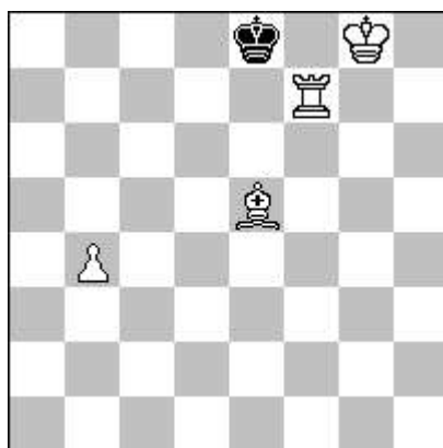
s # 8 Annan (4 + 1)
