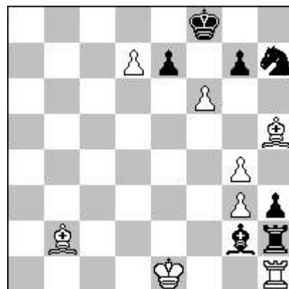
s # 7 (8 + 7)
