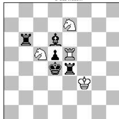
ser-h # 4 2 sol (4 + 5)
