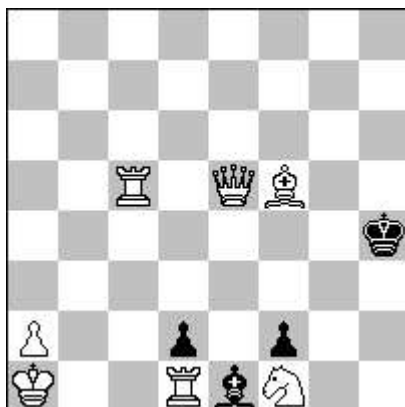
s # 7 2 sol. (7 + 4)
