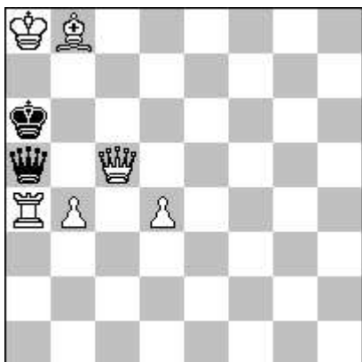
s # 6* (6 + 2)
