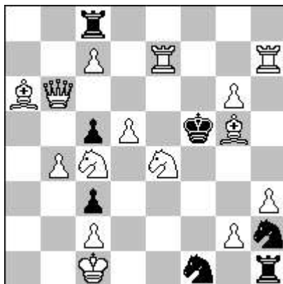
s # 3v (15 + 7)
