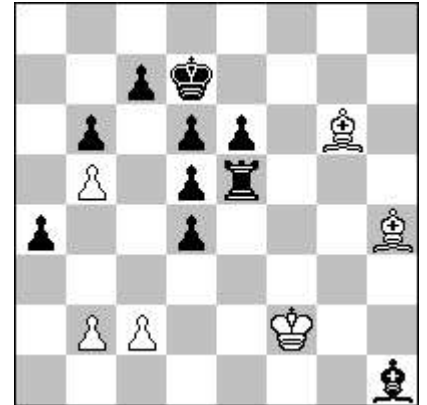
h # 3 b)b5→c4 (6 + 10)
