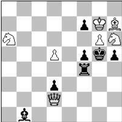
# 4 (7 + 7)
